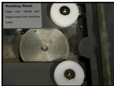
Notching Blade
